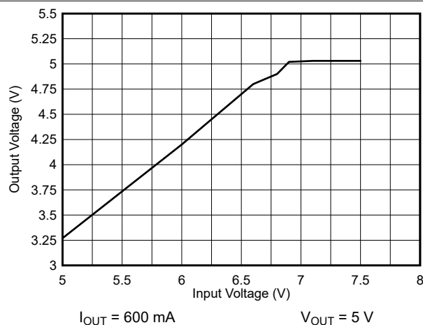
Figure 9-31. Drop-Out Response
