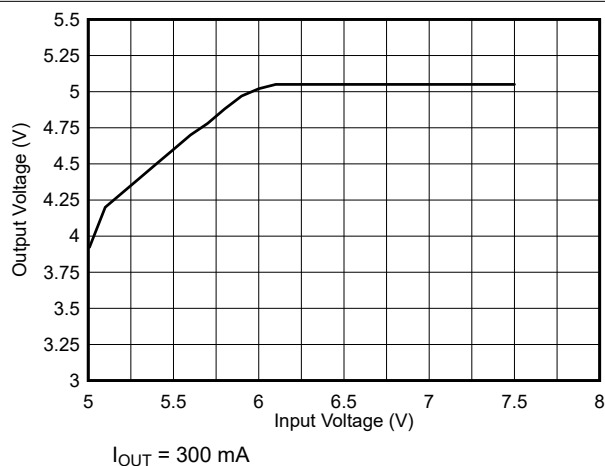
Figure 9-32. Drop-Out Response
