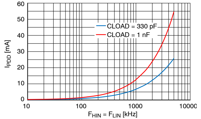
Figure 6. Operating VDD Supply Current ( I_{PDD} ) vs. Frequency ( V_{DD} = 12\text{ V} , SW = PGND , EN = V_{DD} , Both Outputs Switching)
